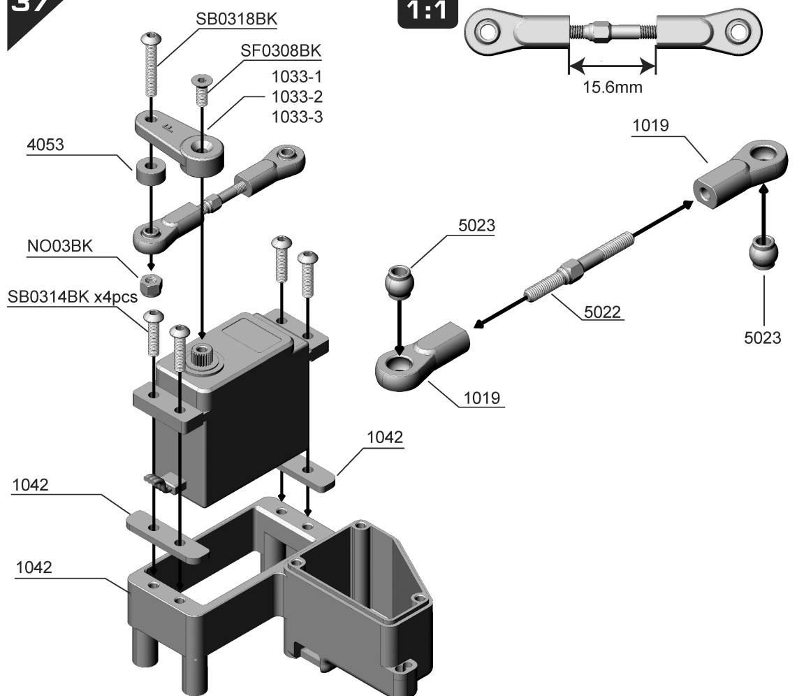
5022 Servo Steering Turnbuckle M3x30mm x 1
