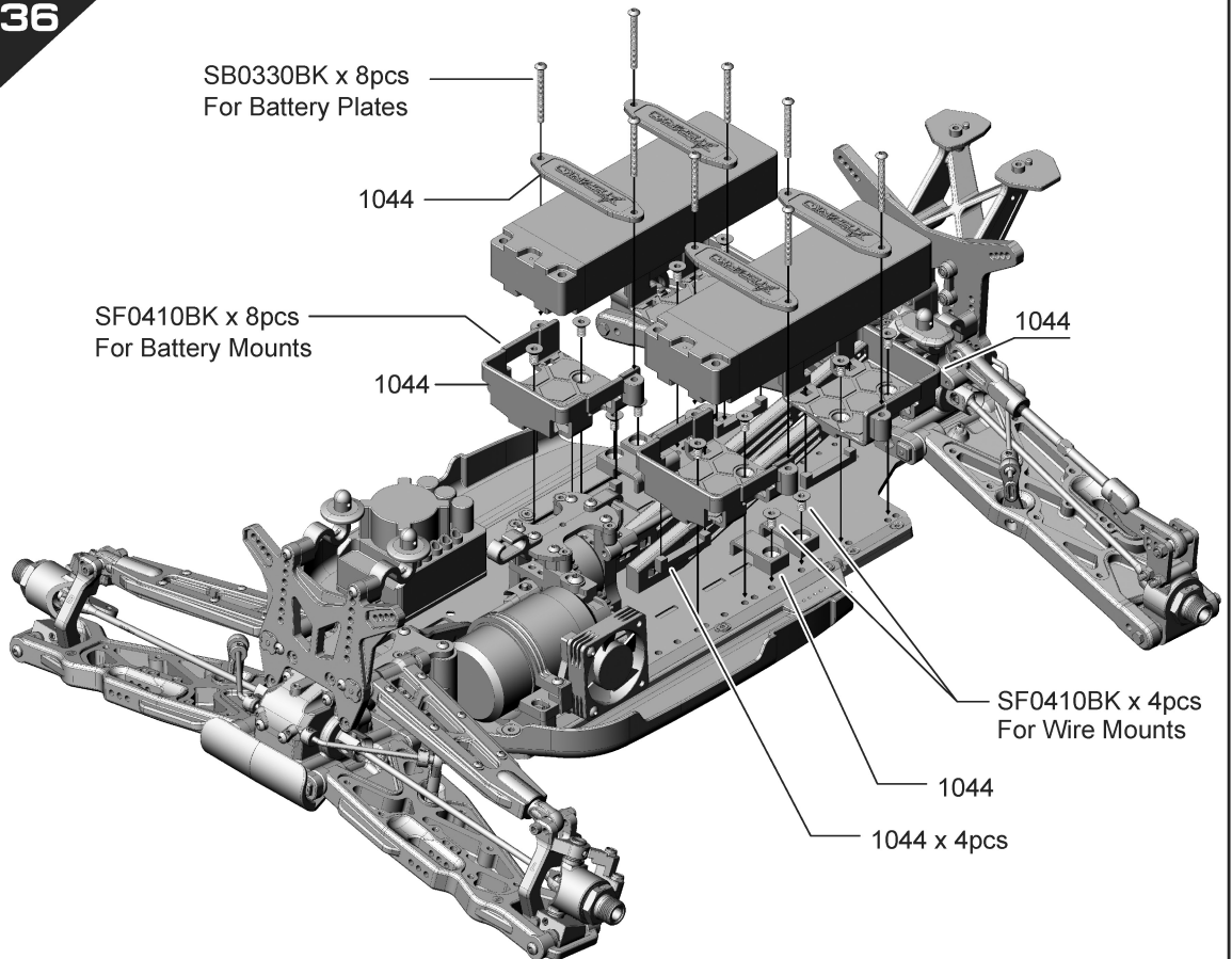
SF0410BK Flat Screw M4x10mm x 12
