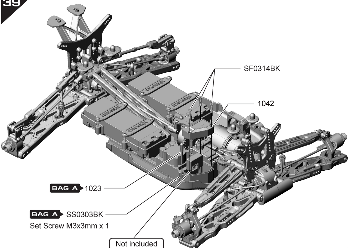
SF0314BK Flat Screw M3x14mm x 3
