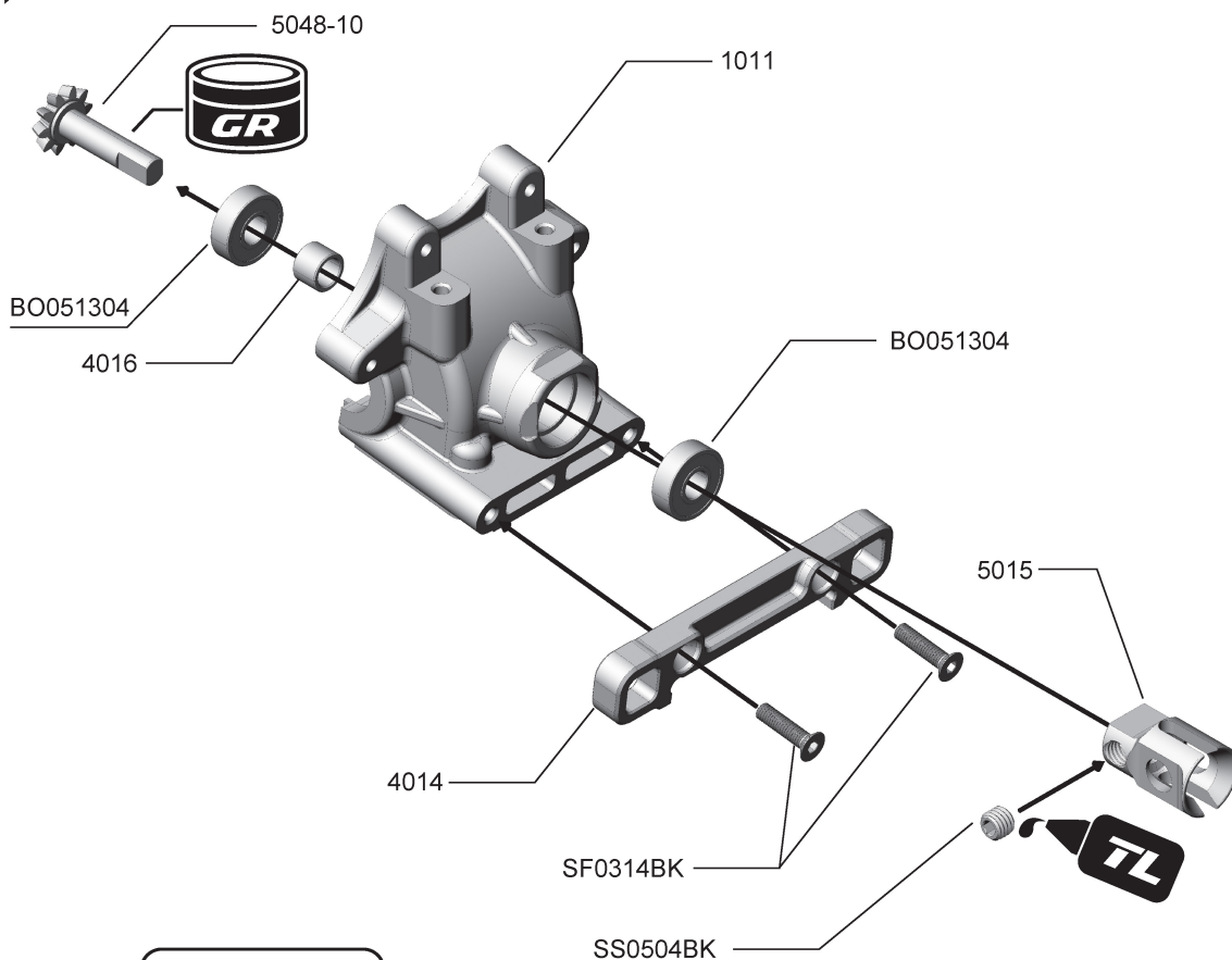
SF0314BK Flat Screw M3x14mm x 2
